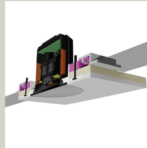
Pre-Construction Flush-Fit
